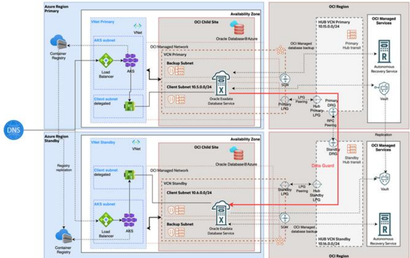
Details of Database Service A based on MAA Reference Architecture 'Gold' across regions
